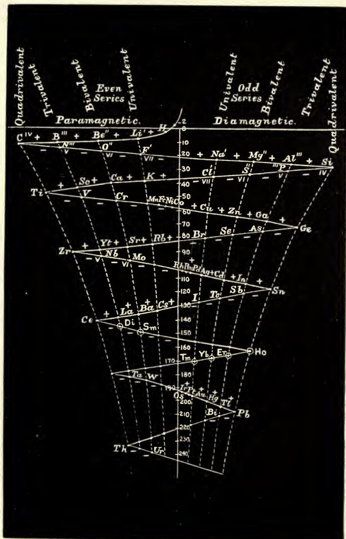
PLATE 7.—Reynolds-Crookes diagram of atomic weights.
